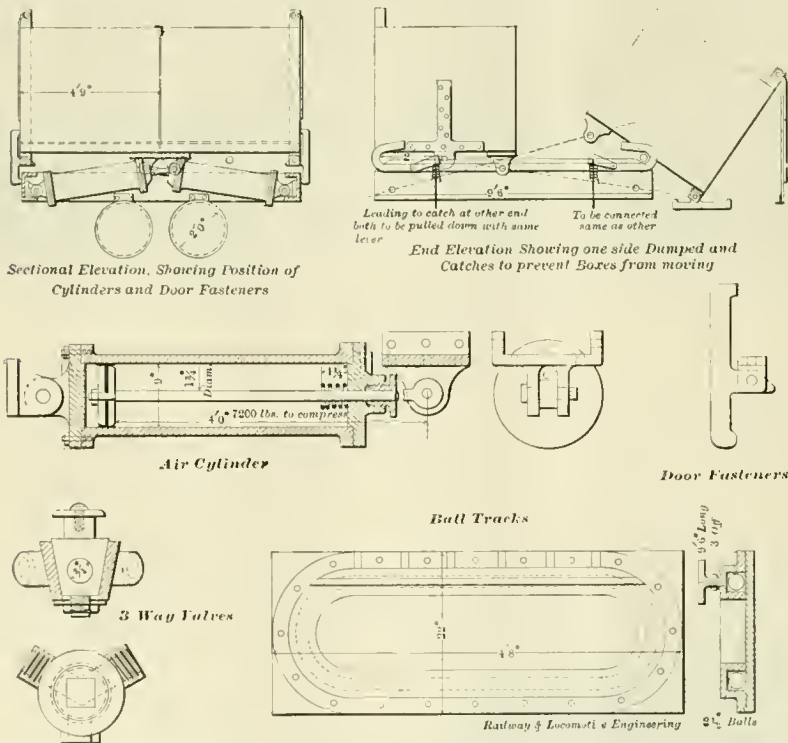
DETAILS OF THE LAWSON IMPROVED DUMPING CAR.
